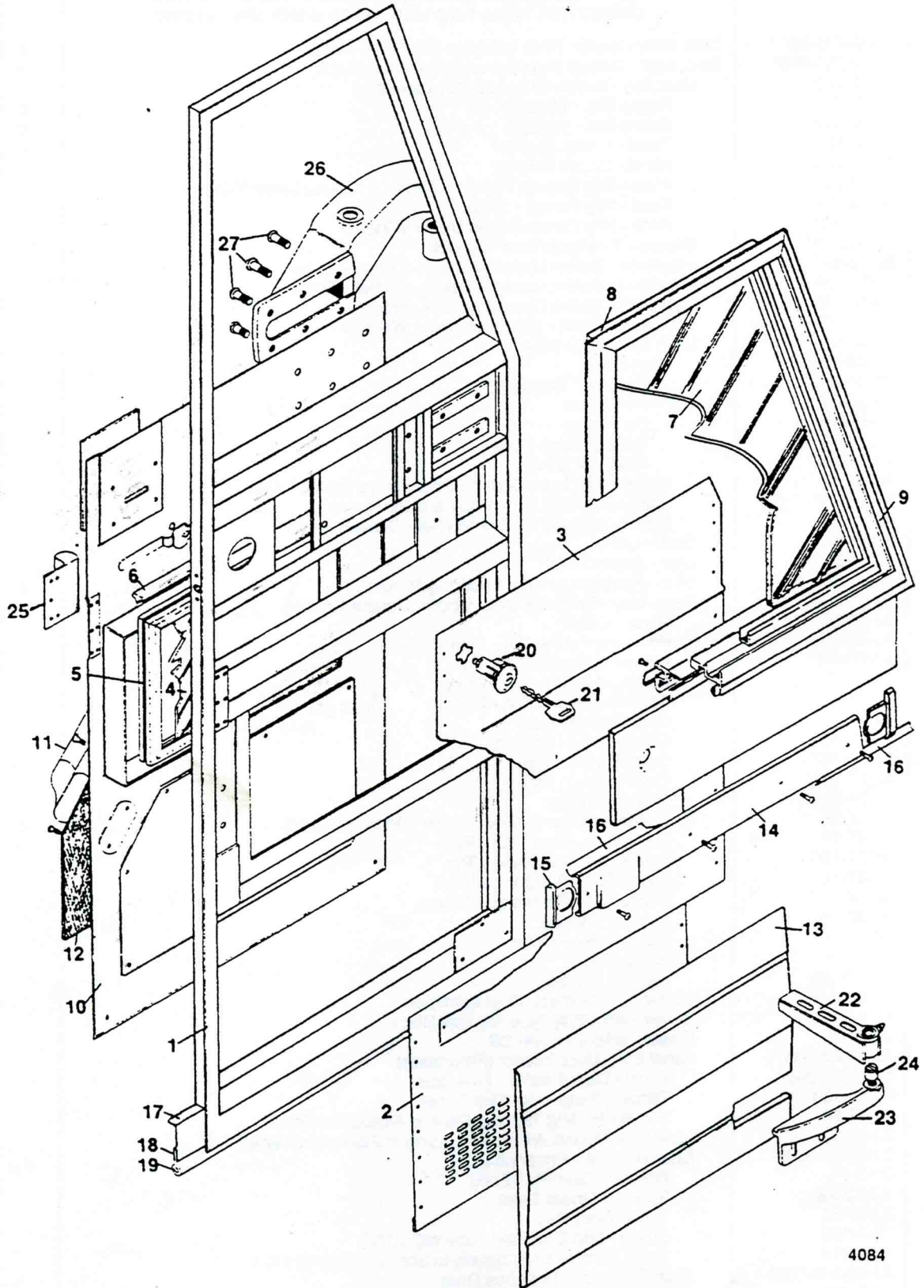
DOOR ASSEMBLY (BASIC) - SEDAN STYLE ENTRANCE (EFFECTIVE WITH TMC UNIT #6855 & MCI UNIT #42492)
